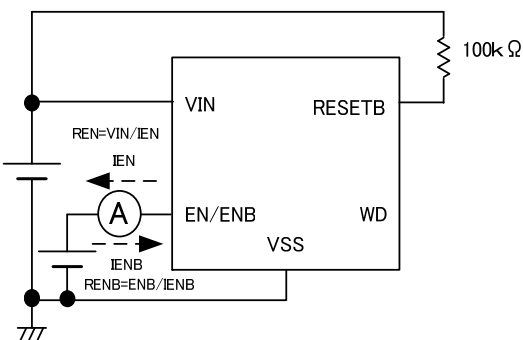
Circuit ⑨
