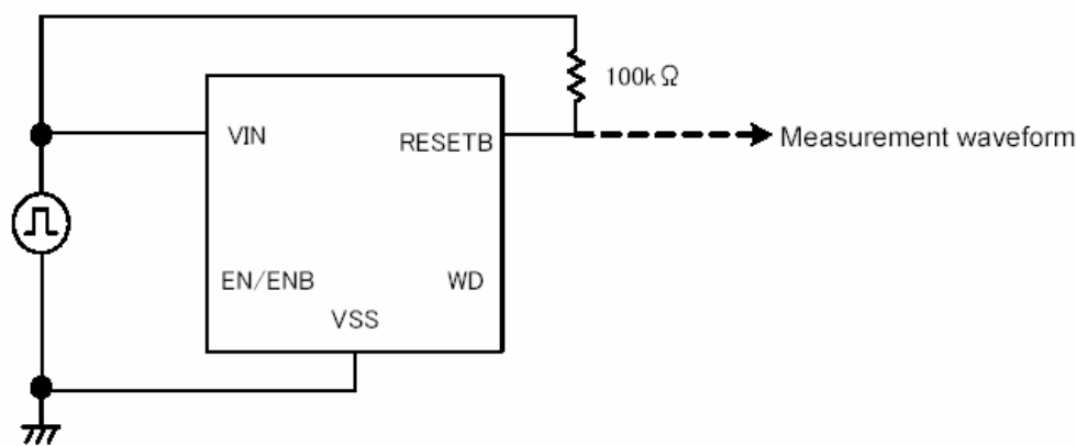
Circuit ④
