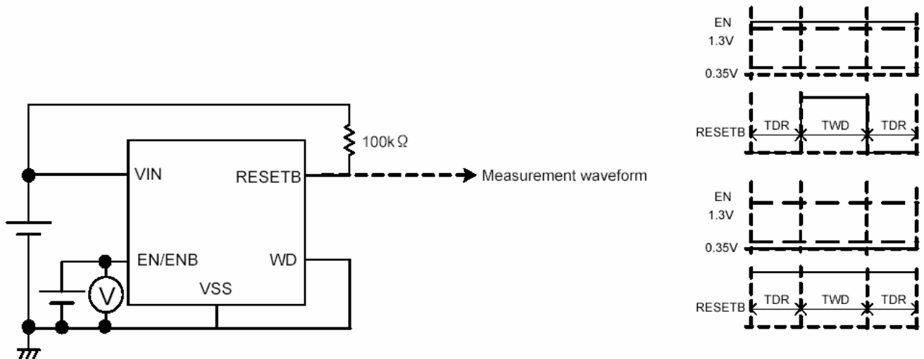
Circuit ⑧
