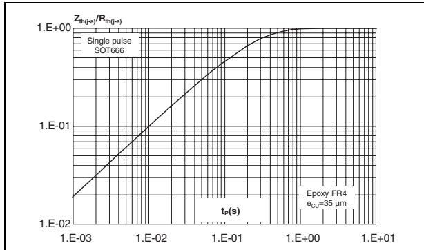
Figure 11. Relative variation of thermal impedance junction to ambient versus pulse duration - epoxy FR4 with recommended pad layout, e_{CU} = 35 \mu\text{m} (SOT-666)
