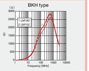
I max=200mA
