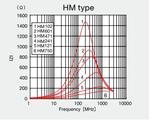
I max=150~350mA
