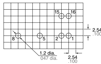
PC board pattern (Copper-side view) DSP1a-PS, DSP1a-PSL2
