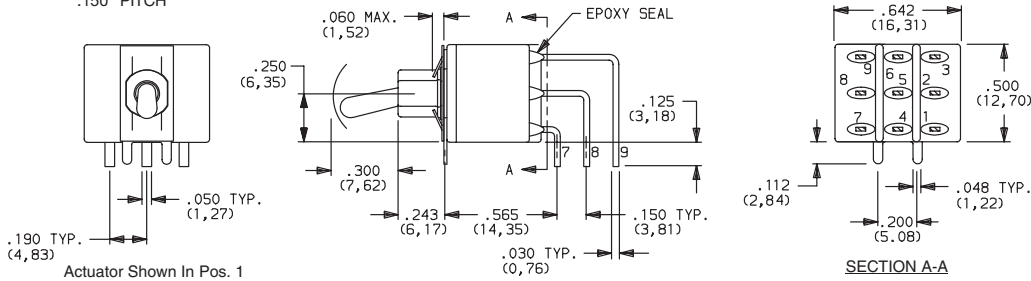
E301MD1AV2BE Vertical Actuation 3PDT
