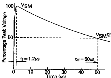
1.2/50µs open-circuit waveform (Haefley Model P6T generator)
