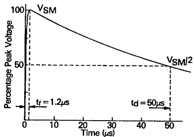
1.2/50µs open-circuit waveform (Haefley Model P6T generator)
