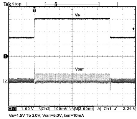
Line Transient
