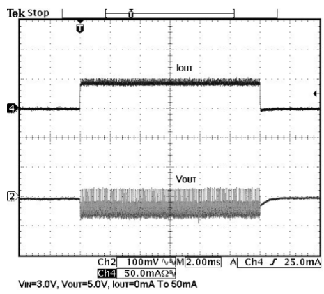
Load Transient
