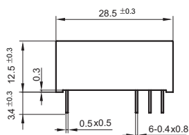
Outline Dimensions
