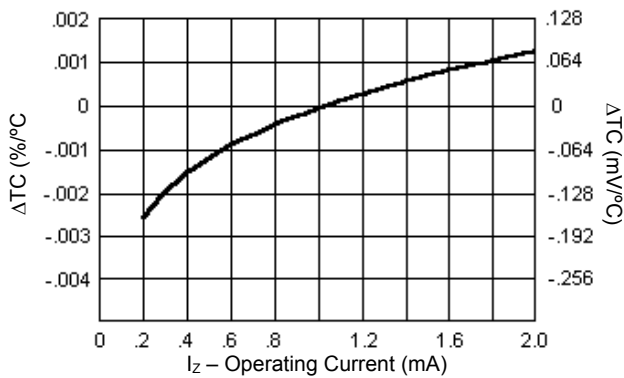
1N4570 – 1N4574A
