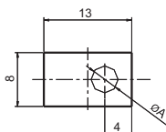
Style 056: A=Ø4.2 Style 056-1: A=Ø5.2
