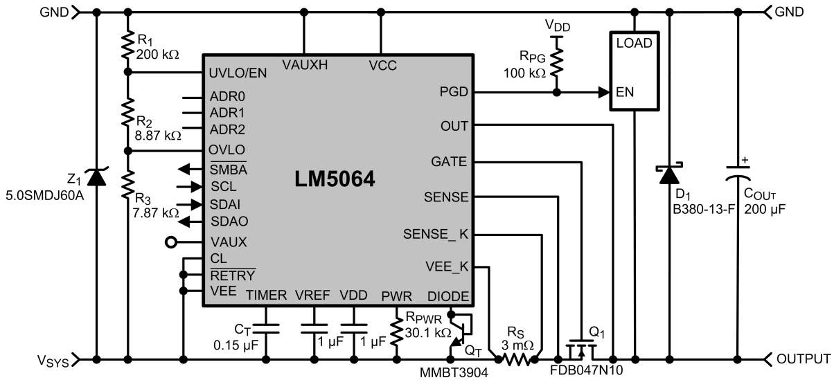
FIGURE 7. Typical Application Circuit
