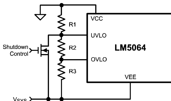
FIGURE 6. Shutdown Control
