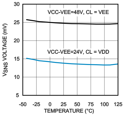
V_{SNS} (SENSE_K-VEE_K) at Power Limit Threshold R_{PWR} = 75\text{ k}\Omega
