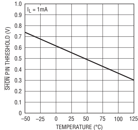
SHDN Pin Threshold (On-to-Off)
