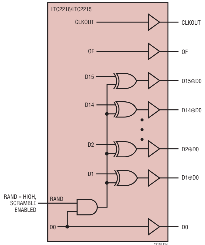
Figure 14. Functional Equivalent of Digital Output Randomizer
