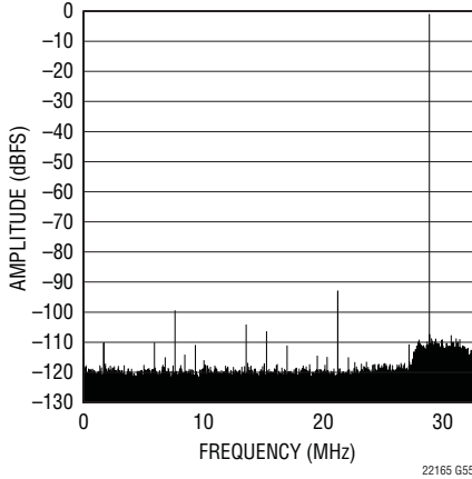
LTC2215 64k Point FFT, f_{IN} = 28.7\text{MHz} , -1dBFS
