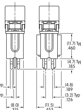
Single Pole
