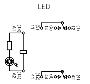
CONNECTION DIAGRAM (BOTTOM VIEW)
