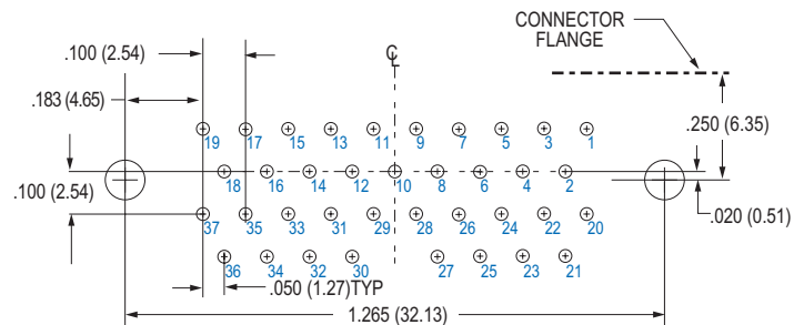
37 SOCKET M83513/13-F
