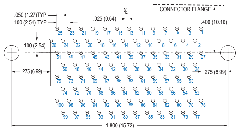
100 SOCKET M83513/15-H
