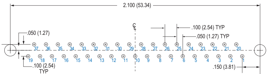
37 PIN M83513/22-F
