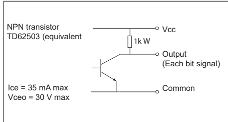
Voltage Output(standard type)
