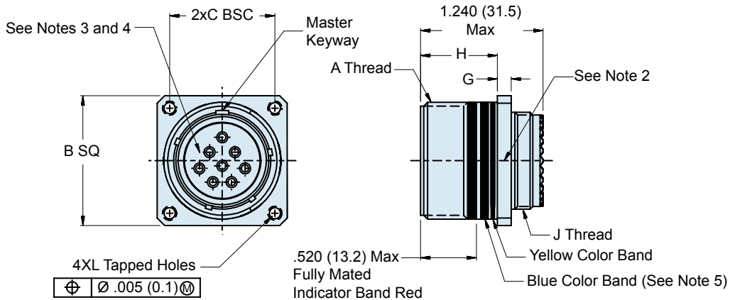
T7 - WALL MOUNT RECEPTACLE SQUARE FLANGE WITH TAPPED HOLES
