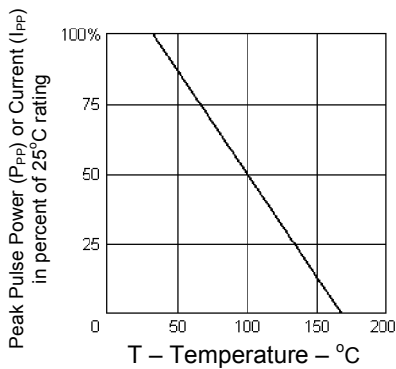
FIGURE 3 DERATING CURVE
