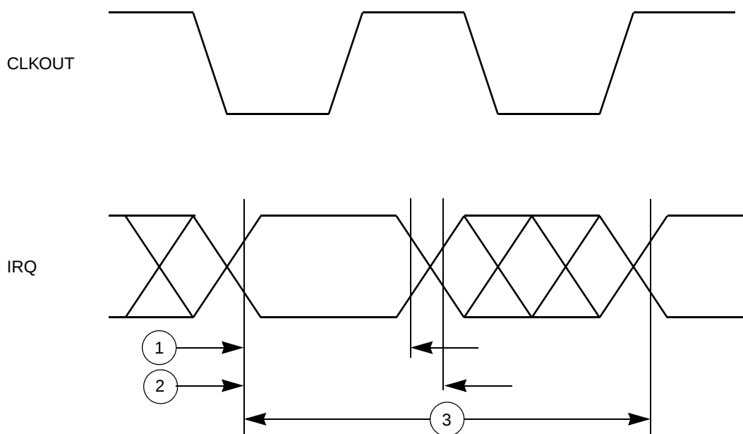
Figure 22. External interrupt timing
