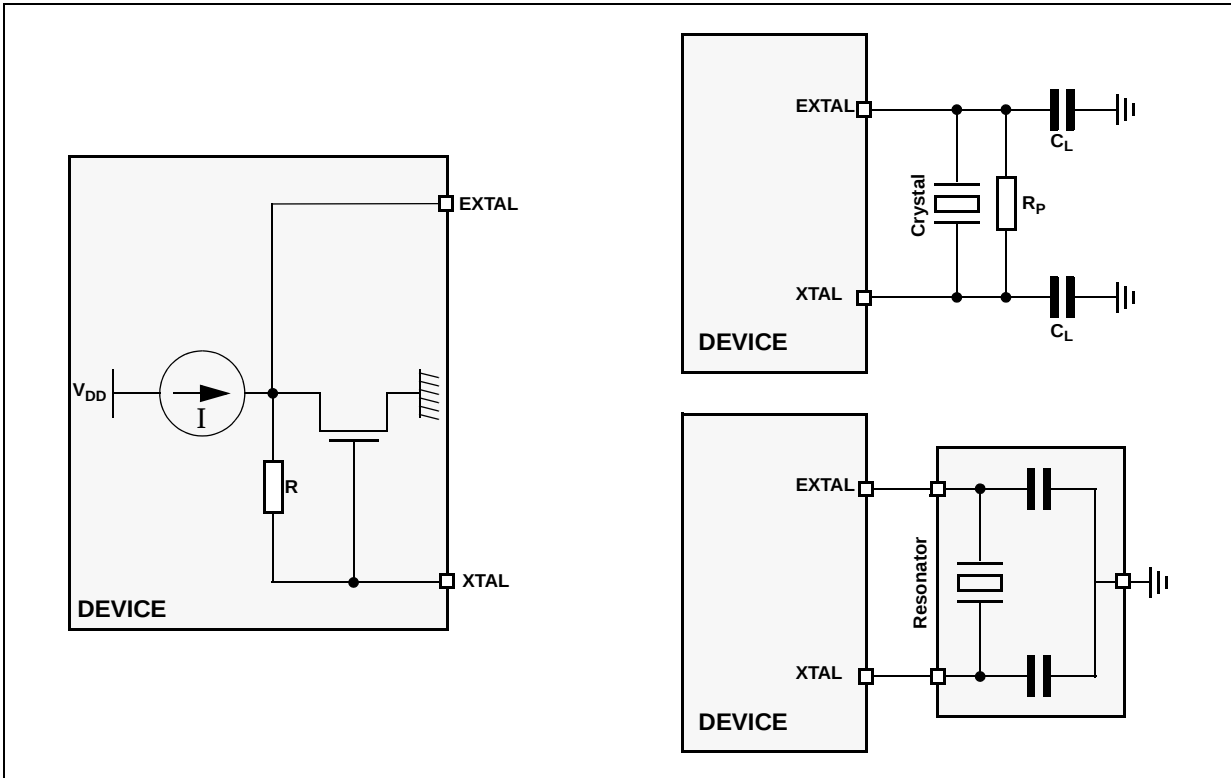
Figure 5. Crystal oscillator and resonator connection scheme
