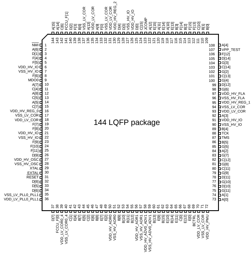
Figure 2. MPC5643L 144 LQFP pinout (top view)
