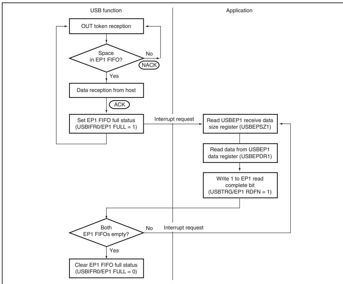
Figure 25.10 EP1 Bulk-OUT Transfer Operation
