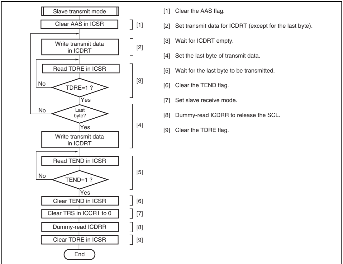
Figure 19.20 Sample Flowchart for Slave Transmit Mode
