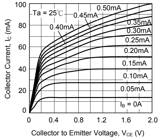
Grounded Emitter Output Characteristics (I)
