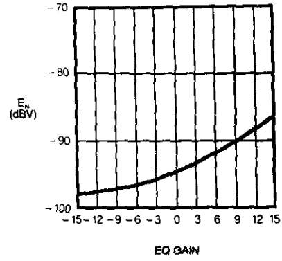
FIGURE 14(B). EQ NOISE PERFORMANCE VS GAIN (20KHz BANDWIDTH)
