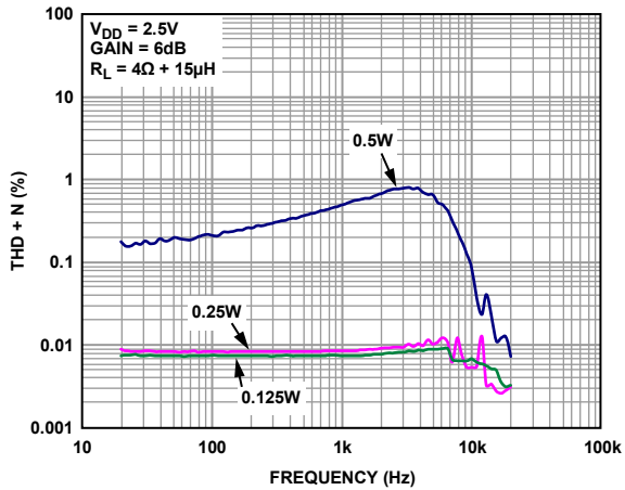
Figure 17. THD + N vs. Frequency, V_{DD} = 2.5V , R_L = 4\Omega , A_v = 6dB
