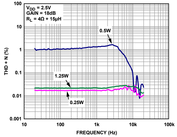
Figure 18. THD + N vs. Frequency, V_{DD} = 2.5V , R_L = 4\Omega , A_v = 18dB
