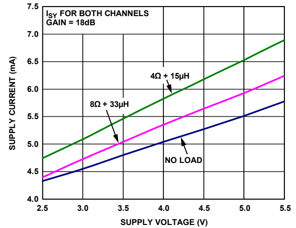
Figure 20. Supply Current vs. Supply Voltage, A_v = 18dB
