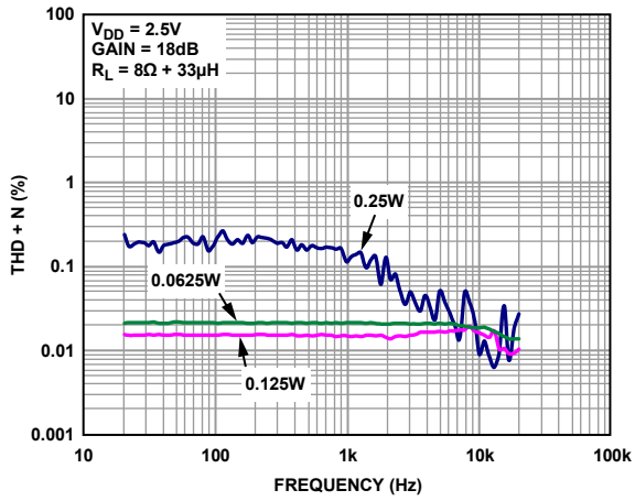
Figure 16. THD + N vs. Frequency, V_{DD} = 2.5V , R_L = 8\Omega , A_v = 18dB
