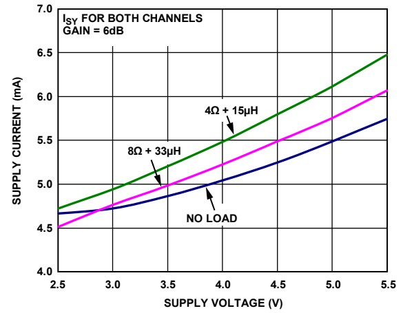
Figure 19. Supply Current vs. Supply Voltage, A_v = 6dB
