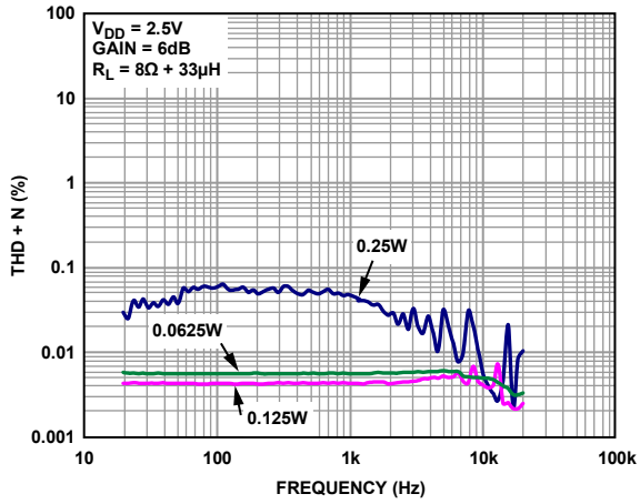
Figure 15. THD + N vs. Frequency, V_{DD} = 2.5V , R_L = 8\Omega , A_v = 6dB
