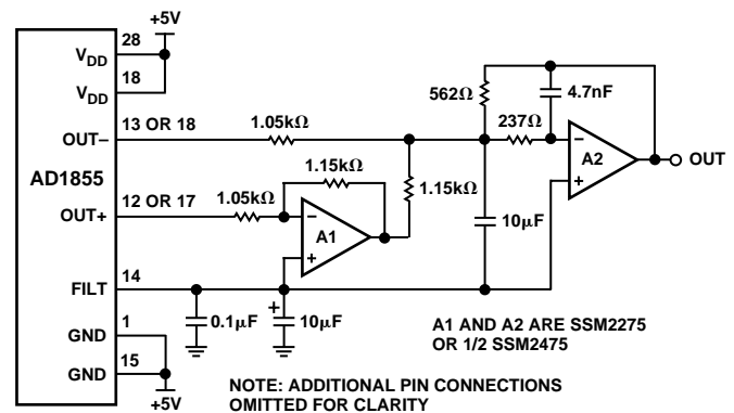
Figure 41. Low-Pass Filter for a 24-Bit Stereo Sigma-Delta DAC
