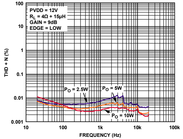
Figure 13. THD + N vs. Frequency; R_L = 4\Omega ; PVDD = 12V; P_O = 2.5W , P_O = 5W , P_O = 10W
