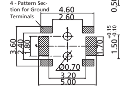
P.C.B. LAYOUT WITH POST
