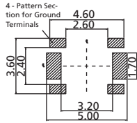
P.C.B. LAYOUT WITHOUT POST
