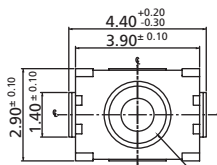
P.C.B. LAYOUT WITH POST
