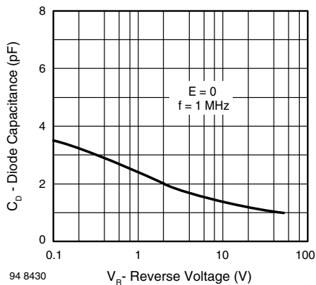
Fig. 1 - Diode Capacitance vs. Reverse Voltage
