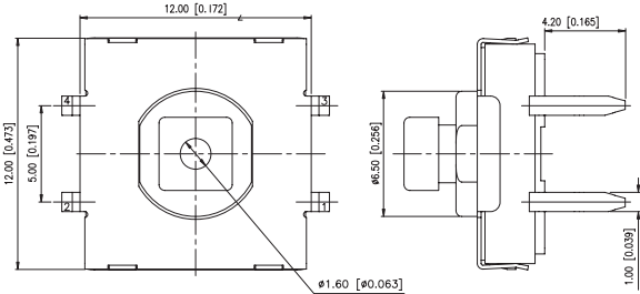
TP57H73: H=7.3
