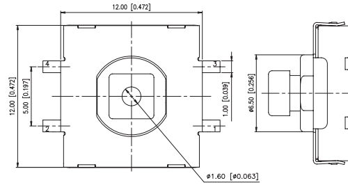
TP57S73: H=7.3
