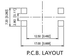
TP57S73: H=7.3
