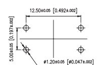
TP57H73: H=7.3
