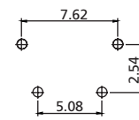
PCB LAYOUT
