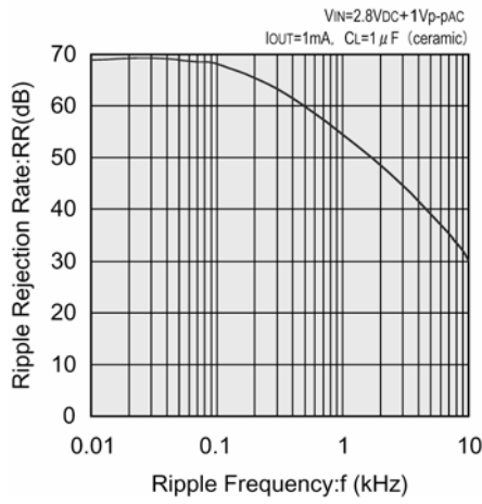
XC6202P182 (1.8V)
