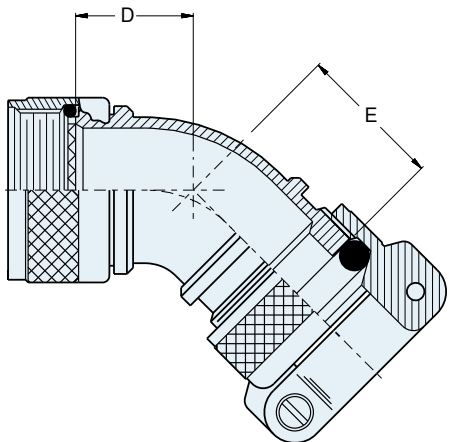
45° ENTRY ROTATABLE COUPLING 370MB038
