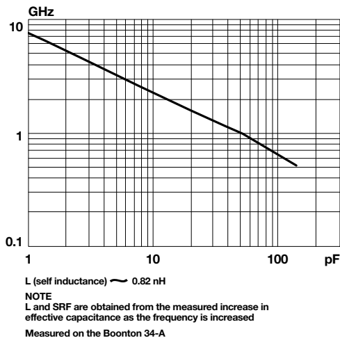
Typical Self Resonant Frequency vs. Capacitance Accu-F ® /Accu-P ® 0805
