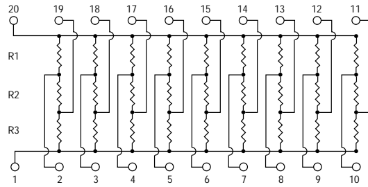
830 ELECTRICAL SCHEMATIC
