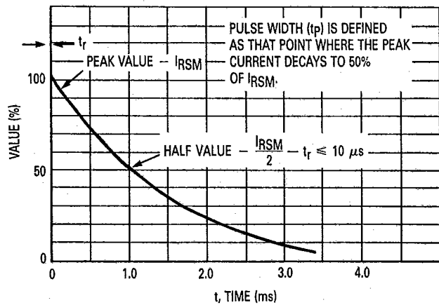
Figure 2. Pulse Waveform
