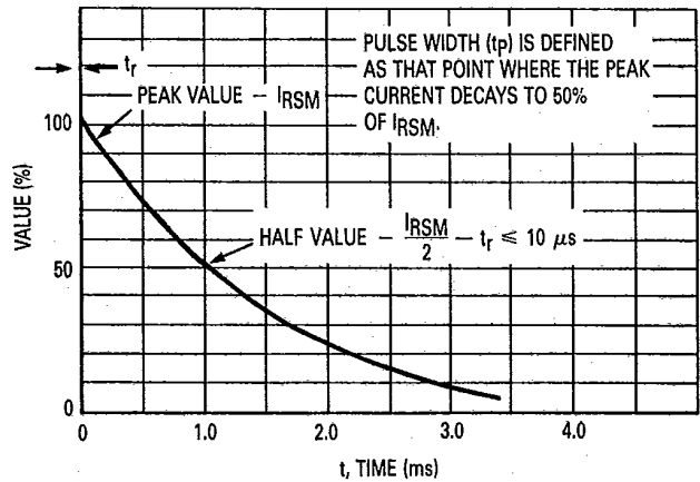
Figure 2. Pulse Waveform
