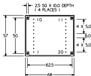
Dimensions, mm
