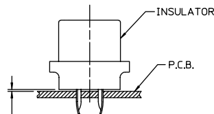
PARTIAL SECTION X-X
