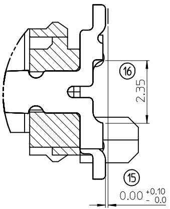
DETAIL 1 SCALE 10:1
